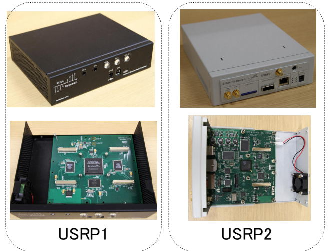
図 4 USRP: Universal Software Radio Periferal
