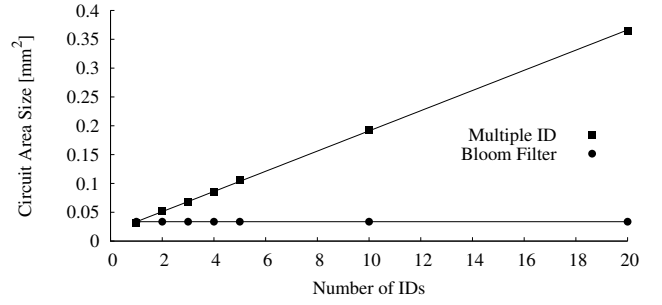
Fig. 8. Circuit area size of the digital circuit.
