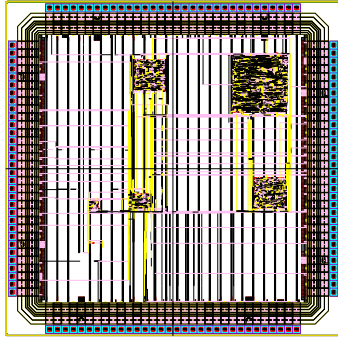
Fig. 7. Chip layout of the digital circuit.
