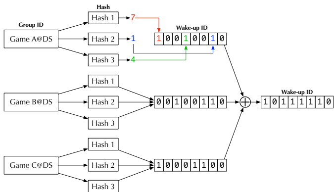
Fig. 3. Process of creating a wake-up ID.
